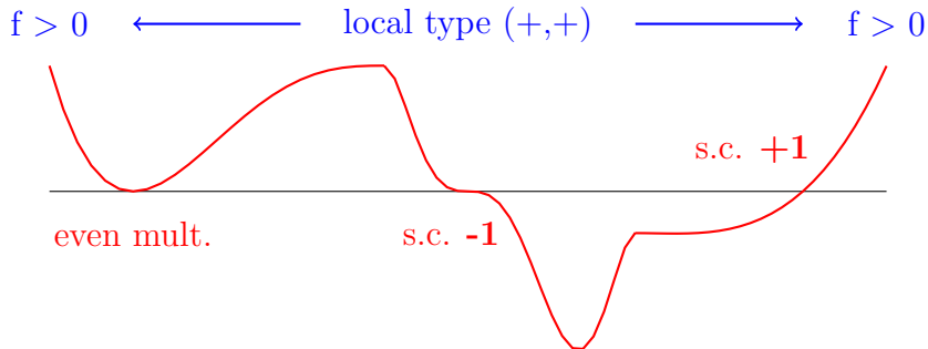
Figure 1: An analytic function f(x) having local type (+, +) in the interval \mathcal{J} .
