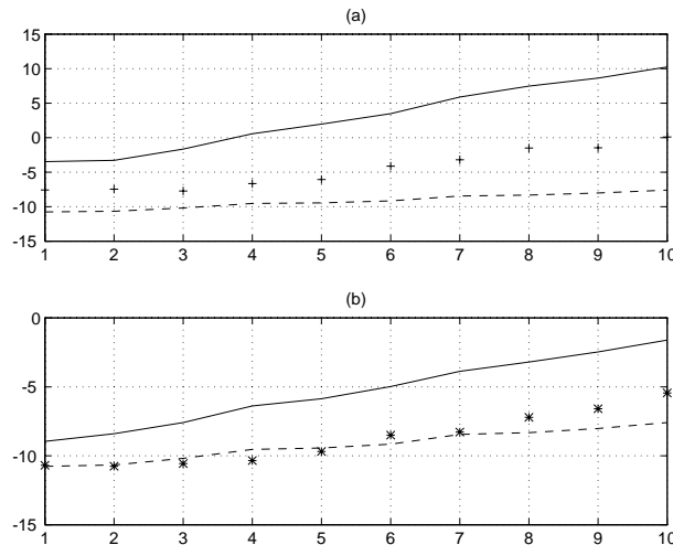
FIG. 2. Error and bounds in Example 3: (a) feedback gain: \log(\|f - \hat{f}\|) : + + +, \log(c_f) : —, \log(eps \cdot \mathcal{S}) : - - -; (b) closed-loop poles: \log(eig_e) : * * *, \log(c_e) : —, \log(eps \cdot \mathcal{S}) : - - -.
